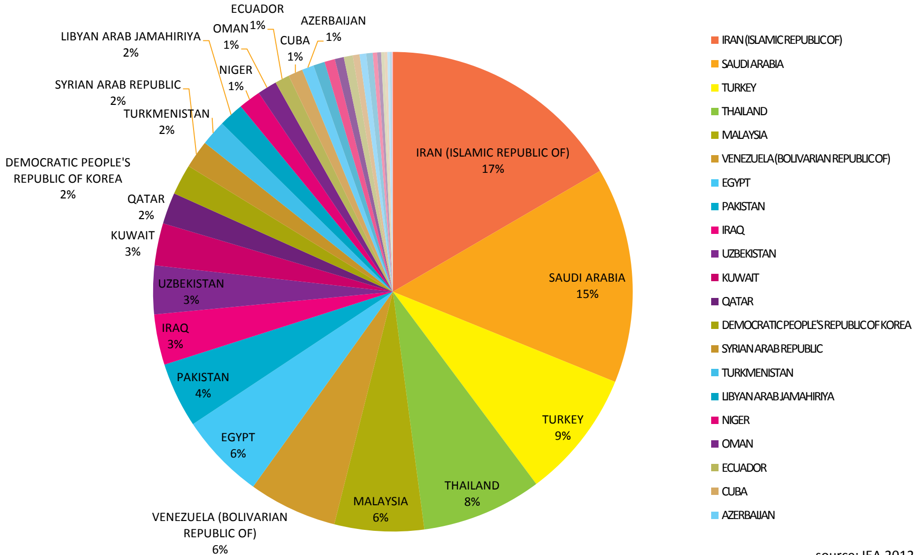
CO2 Emissions(million tonnes of CO2),2010
