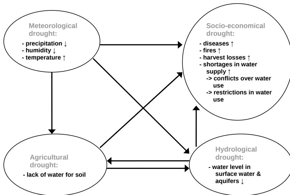
Figure 3: Gradation of drought severity and persistence
